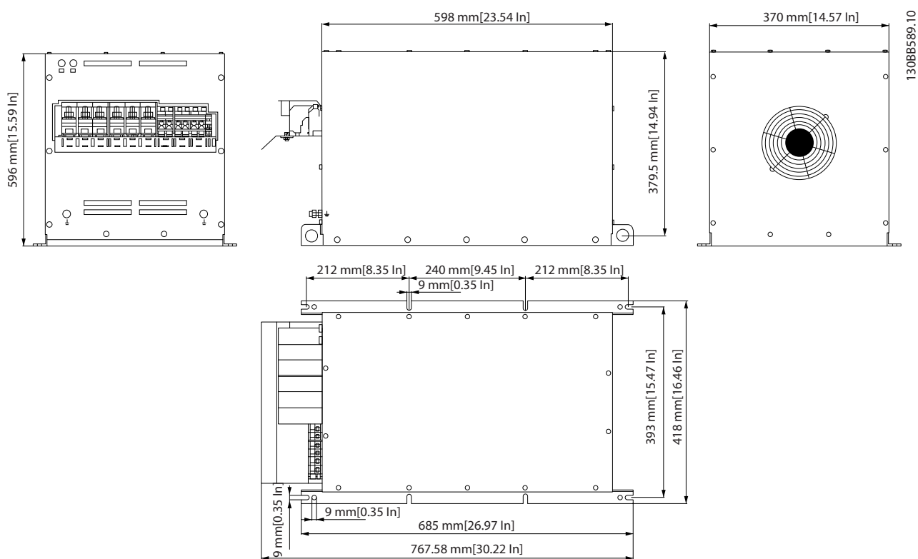
Illustration 6.8 X6 Internal Fan
