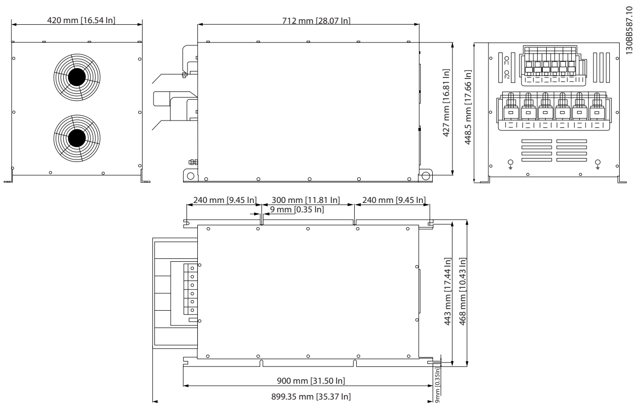
Illustration 6.10 X7 Internal Fan
