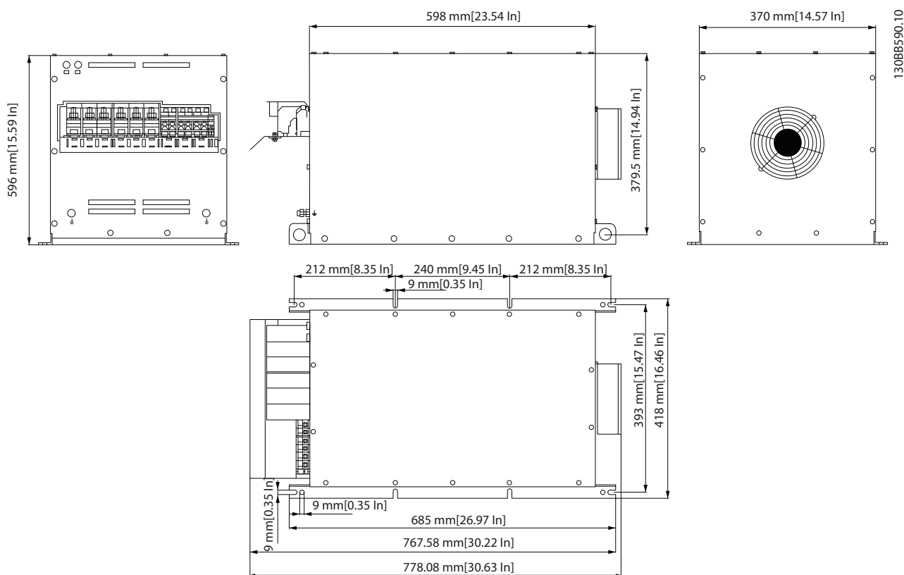
Illustration 6.9 X6 External Fan
