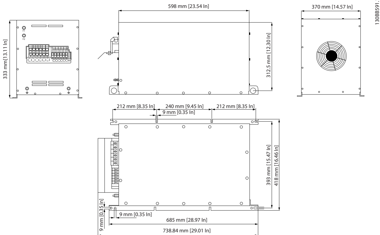
Illustration 6.7 X5 Internal Fan
