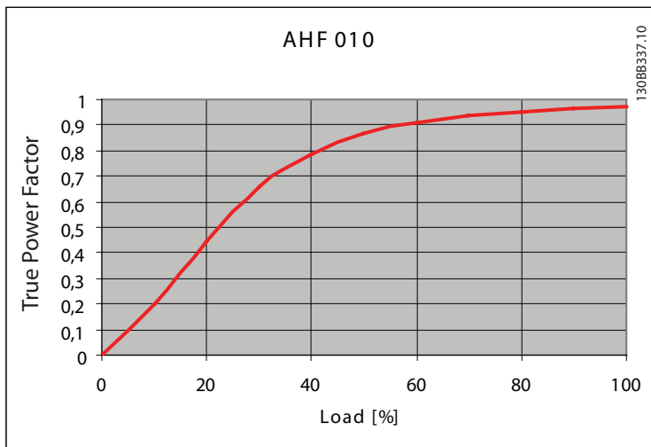
Illustration 4.2: Power Factor as a function of load.
